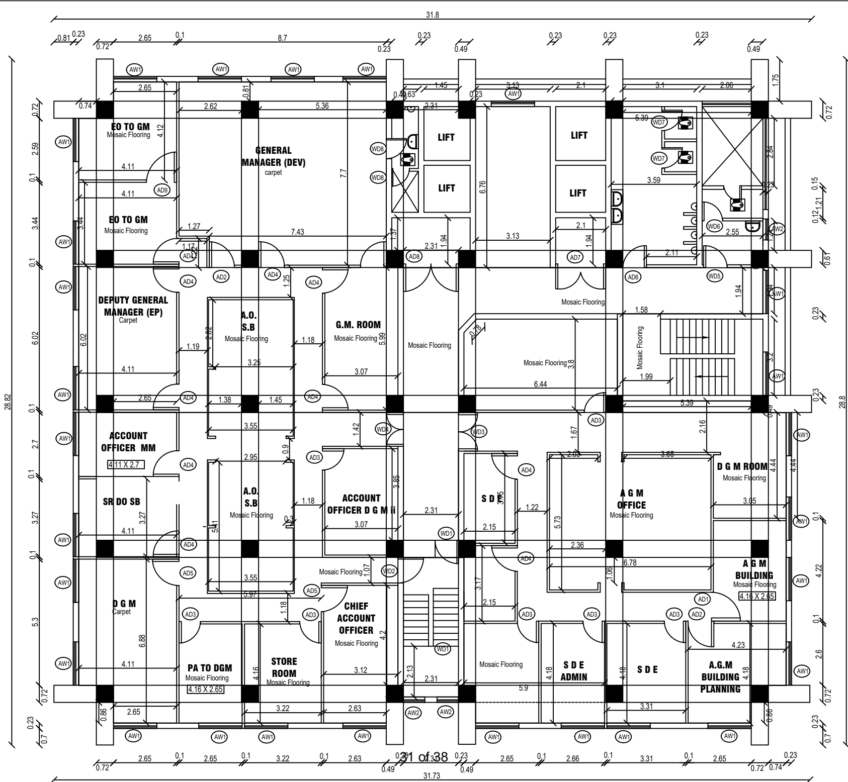
KUSH KUMAR ROAD ADMIN BLDG FOURTH FLOOR PLAN
