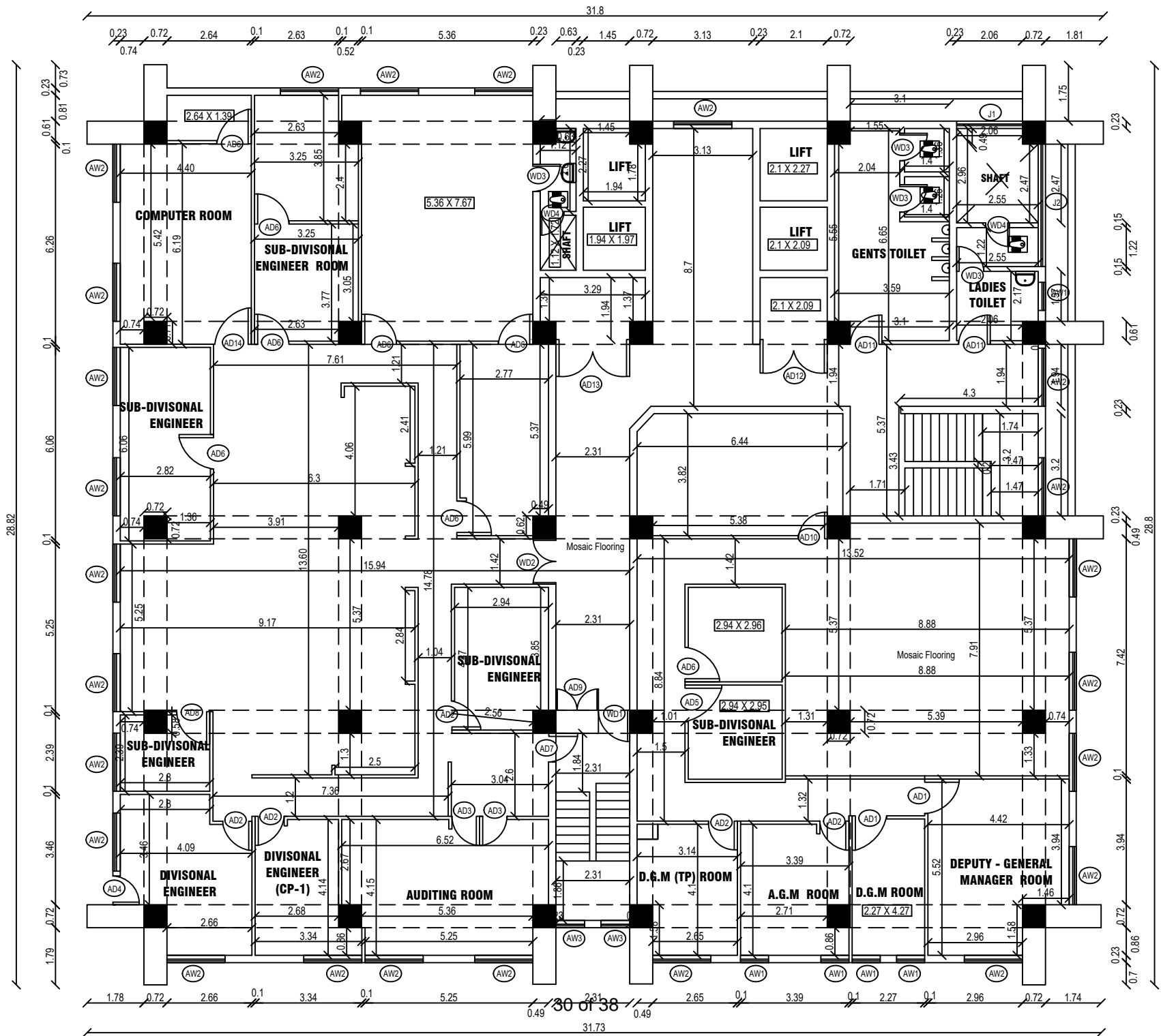
KUSH KUMAR ROAD ADMIN BLDG THIRD FLOOR PLAN
